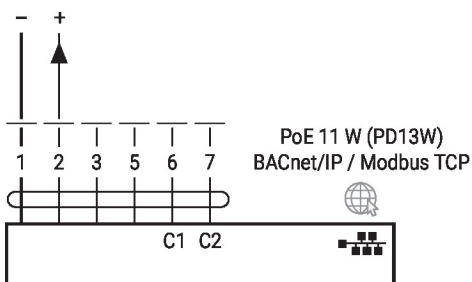
PoE with BACnet/IP / Modbus TCP
