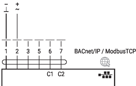
PoE with BACnet/IP / Modbus TCP
