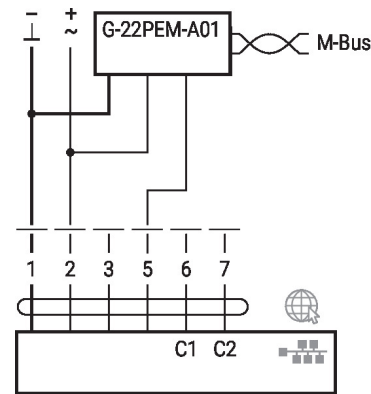
M-Bus with converter in parallel mode with BACnet/IP / Modbus TCP
