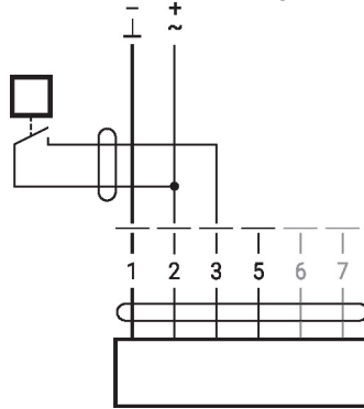
Connection with switching contact
