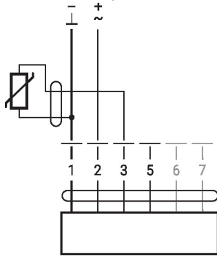
Connection with passive sensor
