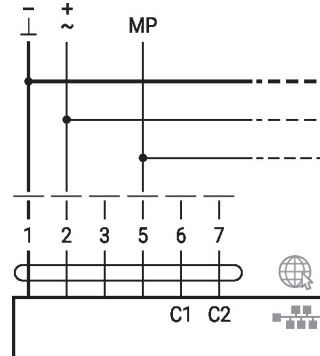
MP-Bus, supply via 3-wire connection
