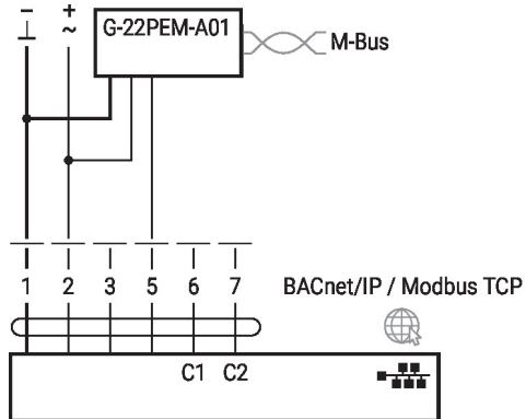
M-Bus with converter in parallel mode with BACnet/IP / Modbus TCP
