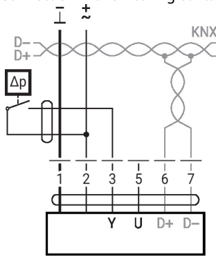
Connection with switching contact, e.g. \Delta p monitor switch
