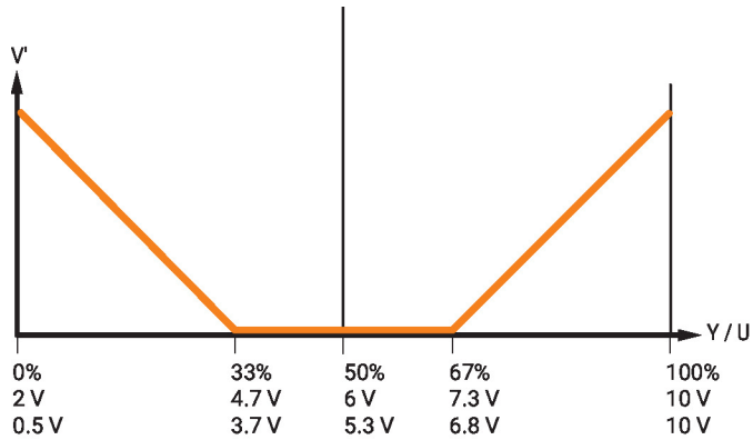
Valve characteristic curve
