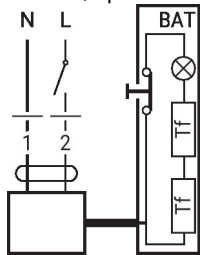
AC 230 V, open/close
