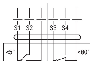
Auxiliary switch
