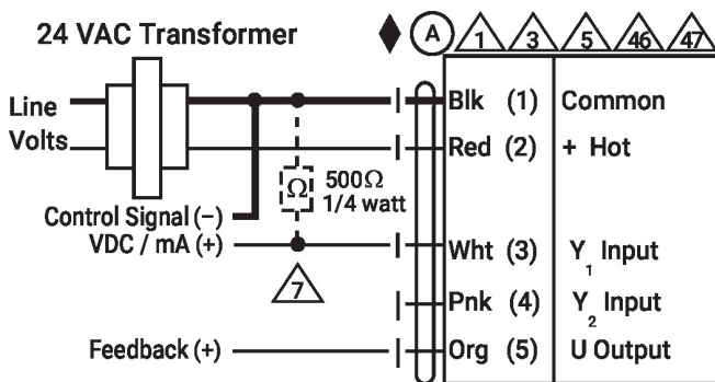
VDC/ma Commande
