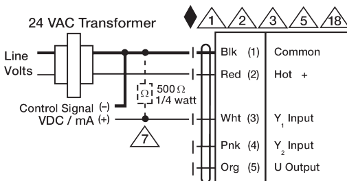
Control VDC/mA
