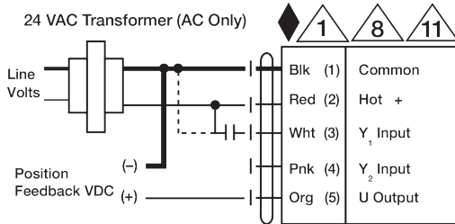
PWM Control
