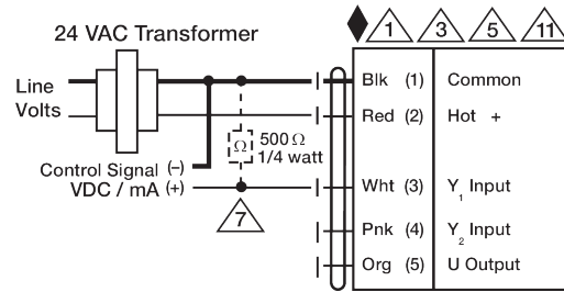
VDC/ mA Control
