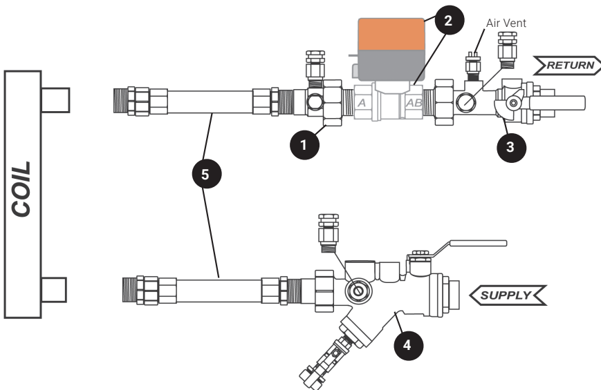
2-way Standard Zone Valve
