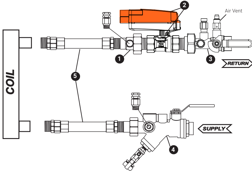
2-way Standard Zone Valve
